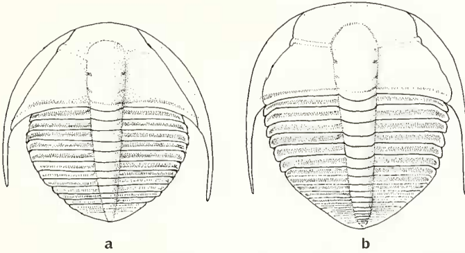
TEXT-FIG. 26. Trinucleaceans crossing the Cambrian-Ordovician boundary. a , Jegoroviaia (Upper Cambrian; after Lu 1974, pl. 2). b , Araiopleura (Tremadoc; after Dean 1970, pl. 1, fig. 11). Both \times 8 approx.
